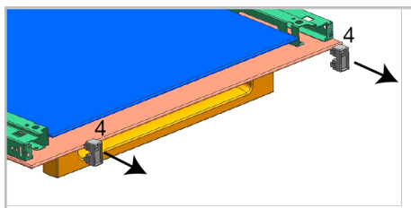
4 Glass holder connecting element*
