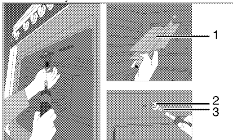
1 Grill burner 2 Injector holder 3 Injector
